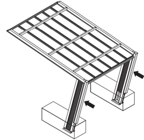
14 Installation of Rainspout Cover
