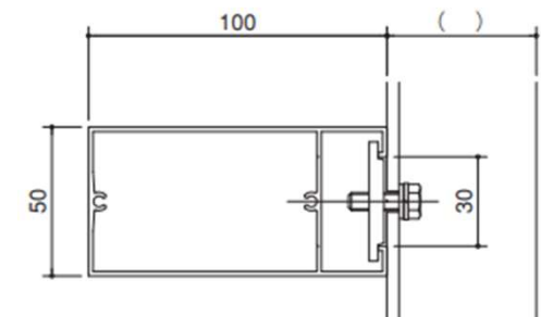
Installation Example
