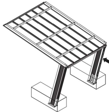
13 Installation of Rainwater Pipe
