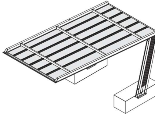
10 Installation of Front Frame Corner Cap
