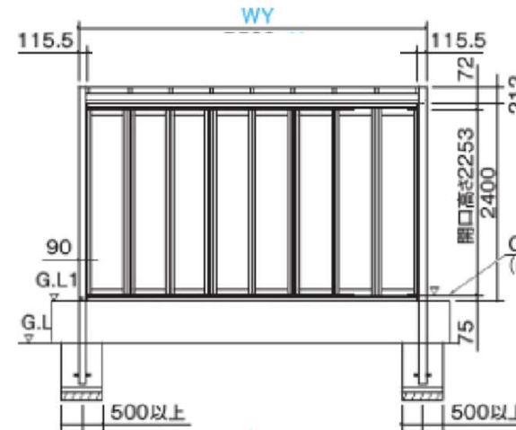
Front side Elevation surface
