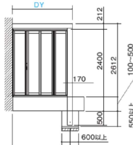
Right and Left Side Elevation surface
