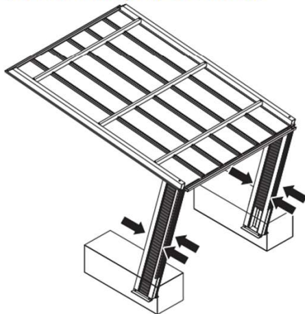
12 Installation of Dress-up Panel•Post Screw Cover•Rainspout Cover Base
